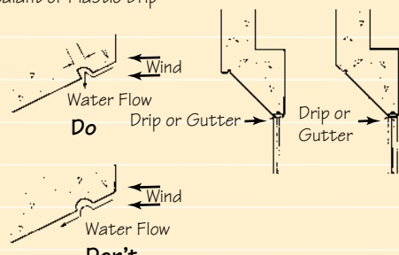
Fig. 10 Drip Details
