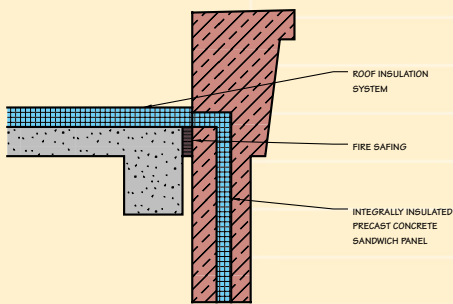
SANDWICH PANEL
