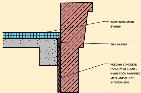
SINGLE WYTHE PANEL
