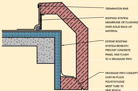
Fig. 3: To prevent leakage, Fencil adds an extra piece of conventional base flashing over the back of panels along the roofline, flashed out at the extended roof membrane beneath the C-shape.
