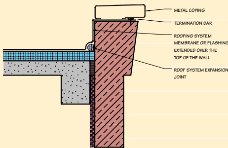
Fig. 2: With a straight-backed cornice panel, Fencil completes the roof detail with a metal, stone or precast coping piece to hide the termination.
